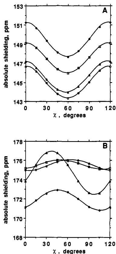
Figure 5. Calculated ^{13}C shieldings as a function of the torsion angle, \chi , for an alanine model fragment at different \phi and \psi angles: (A) C^\alpha shielding for helix ( \phi = -58, \psi = -51 ) (O), turn ( \phi = 55, \psi = 50 ) ( \Delta ), sheet 1 ( \phi = -140, \psi = 140 ) ( \diamond ), and sheet 2 ( \phi = -71, \psi = 140 ) ( \square ); (B) as in A but for (methyl) C^\beta .
