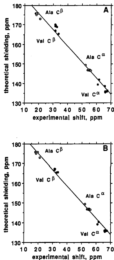
Figure 8. Calculated ^{13}\text{C}^\alpha and ^{13}\text{C}^\beta shieldings for alanine (○) and valine (●) residues in calmodulin: (A) using the torsion angles derived from the X-ray structure, 30 the shielding surfaces shown in Figure 6 for valine, and the alanine shielding surfaces reported in ref 8; (B) as in A but a \chi^1 of 180^\circ is assumed for all valine residues. The experimental chemical shifts are given in ppm from TSP (ref 26).
