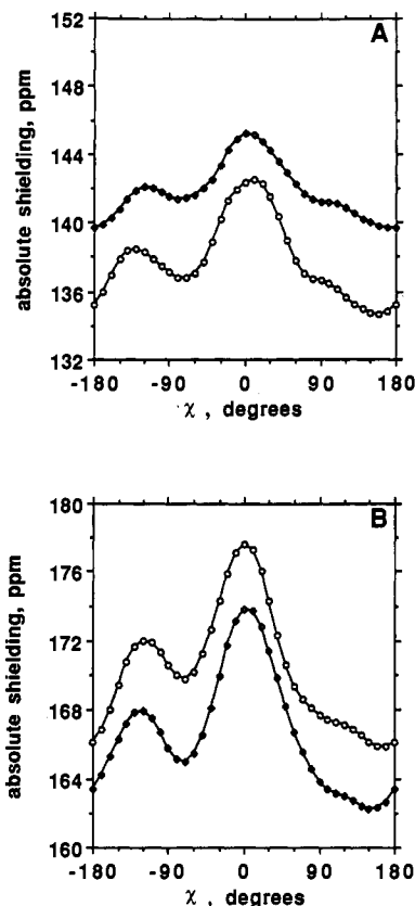
Figure 6. Calculated 13 C shieldings as a function of the torsion angle, \chi , for a valine model fragment at different \phi and \psi angles: (A) C \alpha shielding for helix ( \phi = -55^\circ, \psi = -55^\circ ) (O) and sheet ( \phi = -136^\circ, \psi = 143^\circ ) ( \diamond ); (B) as in A but for C \beta .
